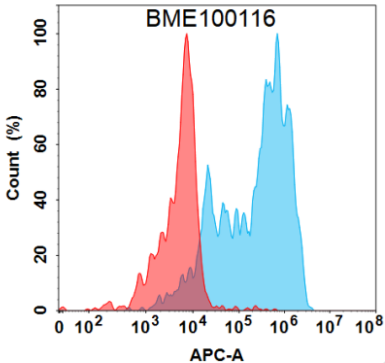
Figure 2. Flow cytometry analysis under cell membrane permeable condition with 1 \mu\text{g}/\text{mL} Anti-IL1B (canakinumab biosimilar) mAb (BME100116) on HEK293 cells transfected with Human IL1B protein (Blue histogram) or HEK293 transfected with irrelevant protein (Red histogram).
