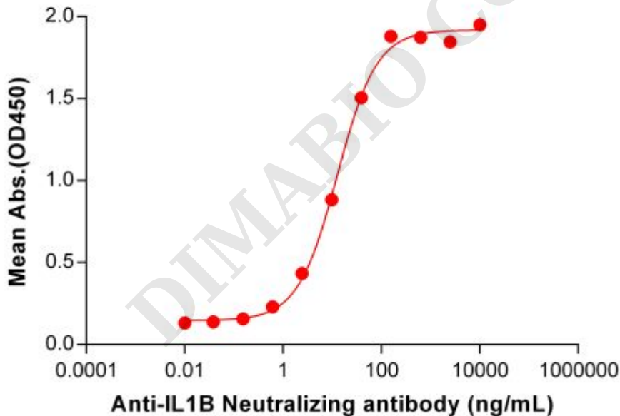
Figure 1. ELISA plate pre-coated by 1 µg/mL (100 µL/well) Human IL1B Protein, hFc Tag (PME100838) can bind Anti-IL1B Neutralizing antibody (BME100116) in a linear range of 0.61-156.25 ng/mL. In order to specifically detect BME100116, mouse anti-human Fab-specific antibody was used as detection antibody.
