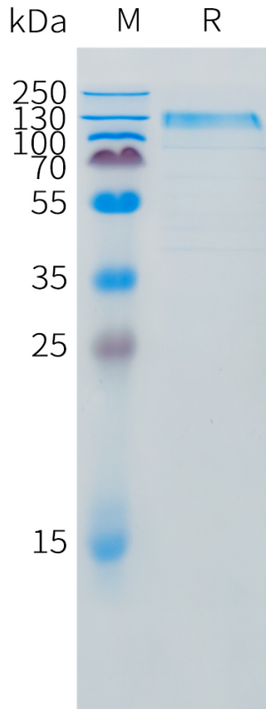
Figure 1. Canine IL31RA Protein, mFc Tag on SDS-PAGE under reducing condition.
