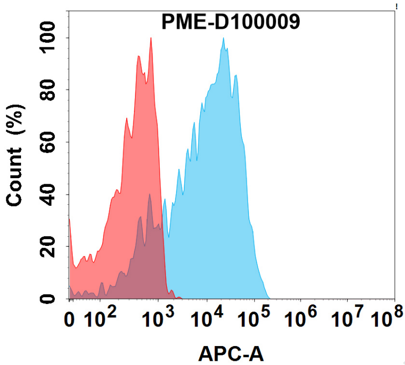
Figure 3. Flow cytometry analysis with 1 \mu g/mL Canine PD-L1 Protein, hFc Tag(PME-D100009) on HEK293 cells transfected with Canine PD-1 protein (Blue histogram) or HEK293 transfected with irrelevant protein (Red histogram).
