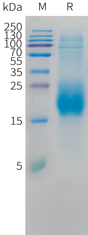
Figure 1. Cynomolgus CD3D Protein, His Tag on SDS-PAGE under reducing condition.
