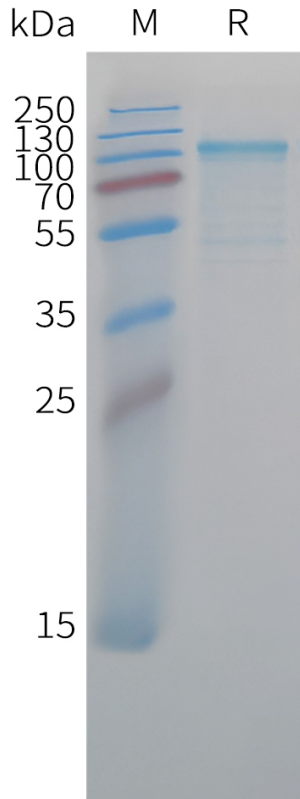
Figure 1. Cynomolgus CDH6 Protein, His Tag on SDS-PAGE under reducing condition.
