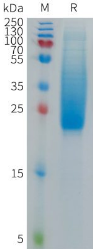
Figure 1. Cynomolgus IL18BP Protein, His Tag on SDS-PAGE under reducing condition.
