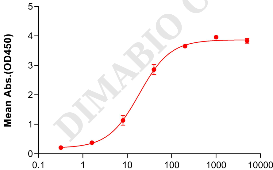
Figure 2. ELISA plate pre-coated by 2 µg/mL (100 µL/well) Human CCR6 Protein, mFc Tag (PME101105) can bind Anti-CCR6 antibody(DMC477); IgG1 Chimeric mAb (DMC100477) in a linear range of 8-40 ng/mL.
