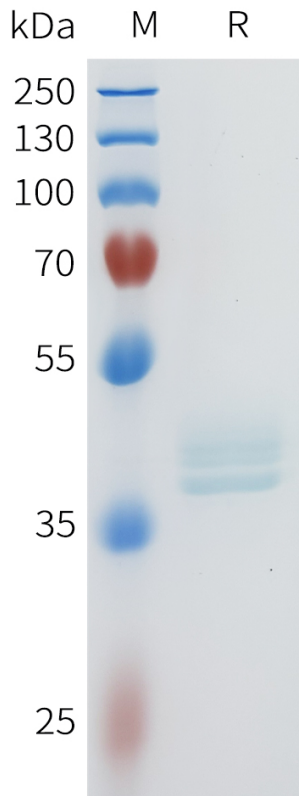
Figure 1. Human CD117(26-120) Protein, hFc Tag on SDS-PAGE under reducing condition.
