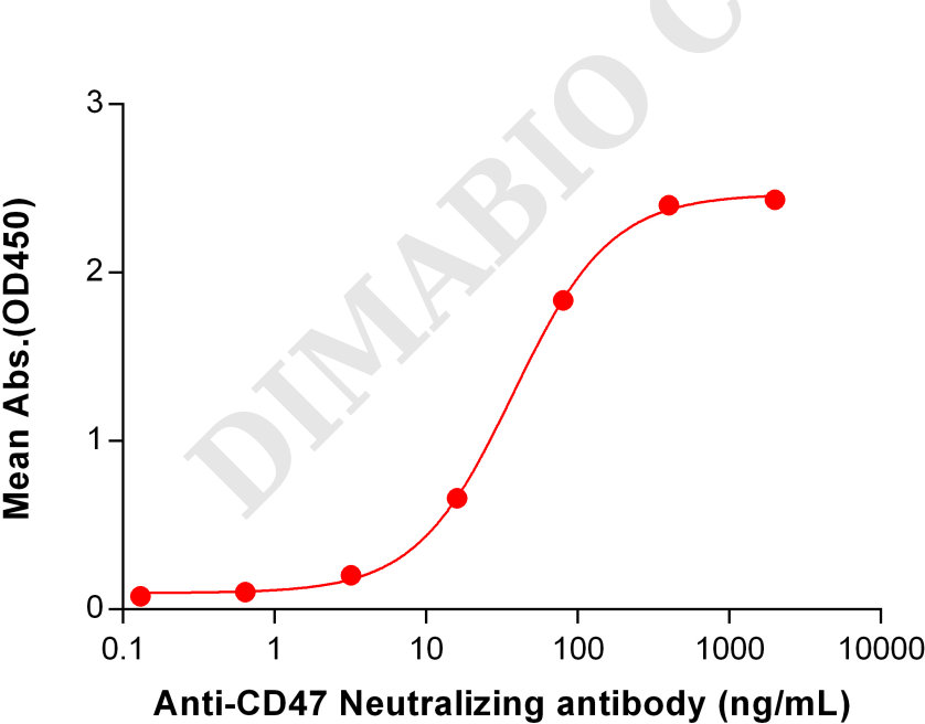
Figure 4. ELISA plate pre-coated by 1 µg/ml (100 µl/well) Human CD47, mFc-His tagged protein (PME100008) can bind Anti-CD47 Neutralizing antibody BME100050 in a linear range of 3.2-80.0 ng/ml.
