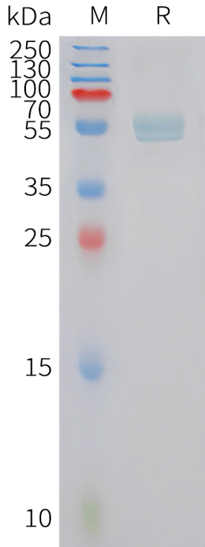
Figure 1. Human CLEC7A Protein, hFc Tag on SDS-PAGE under reducing condition.
