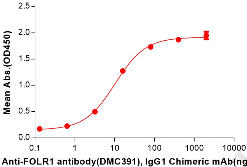
Figure 2. ELISA plate pre-coated by 2 \mu g/mL (100 \mu L/well) Human FOLR1 Protein, His Tag (PME100249) can bind Anti-FOLR1 antibody(DMC391), IgG1 Chimeric mAb in a linear range of 3.20-80 ng/mL.
