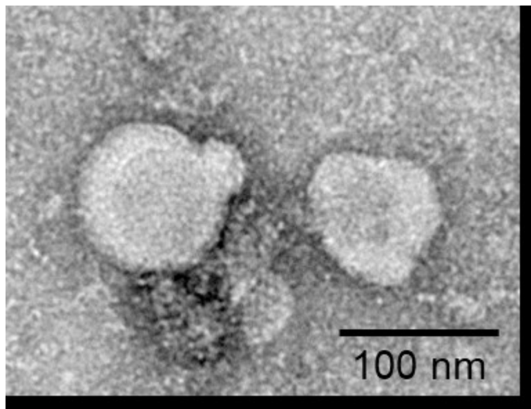
Figure3. TEM image of GPRC5D exosomes
