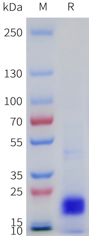
Figure 1. Human IL33(109-270) Protein, N-His Tag on SDS-PAGE under reducing condition.
