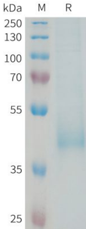
Figure 1. Human KIR3DL3 Protein, His Tag on SDS-PAGE under reducing condition.
