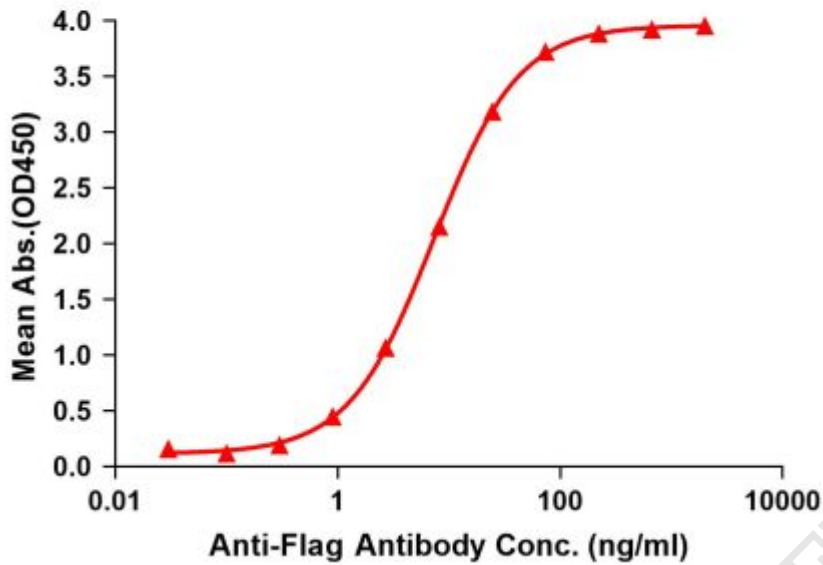
Figure1. Elisa plates were pre-coated with Flag Tag OR1E1-Nanodisc (0.2 \mu g/per well). Serial diluted anti-Flag monoclonal antibody solutions were added, washed, and incubated with secondary antibody before Elisa reading. From above data, the EC50 for anti-Flag monoclonal antibody binding with OR1E1-Nanodisc is 7.304ng/ml.
