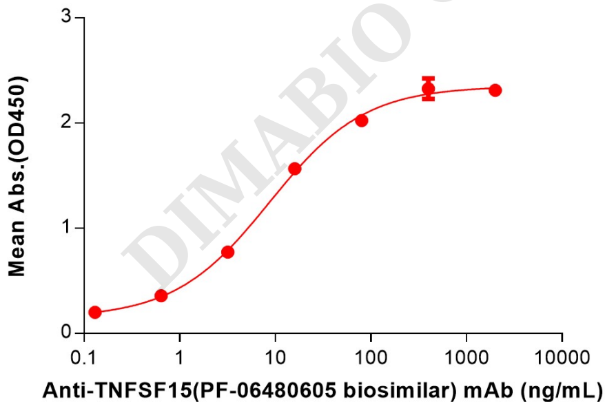
Figure 2. ELISA plate pre-coated by 2 \mu g/mL (100 \mu L/well) Human TNFSF15 Protein, hFc Tag (PME100752) can bind Anti-TNFSF15(PF-06480605 biosimilar) mAb (BME100222) in a linear range of 0.64–80 ng/mL.
