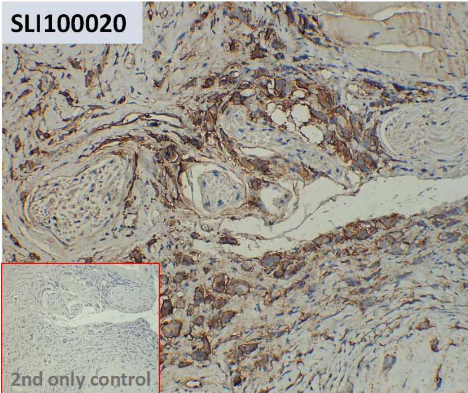
Figure 1. IHC analysis of M-NSG T47-D DiSliceX™ SlideSet section (Cat. No. SLI100020) with anti-TROP2 antibody at a concentration of 10 µg/ml. The inset image shows the absence of staining in secondary antibody-only control.
