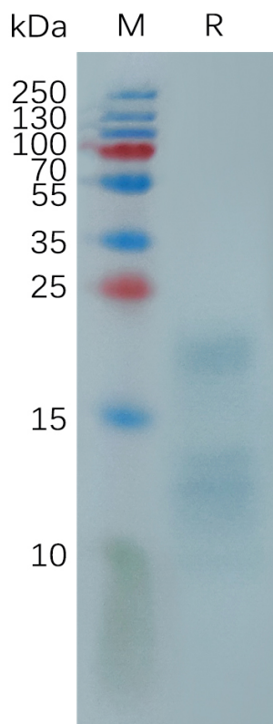
Figure 1. Monkeypox virus A29L Protein, His Tag on SDS-PAGE under reducing condition.
