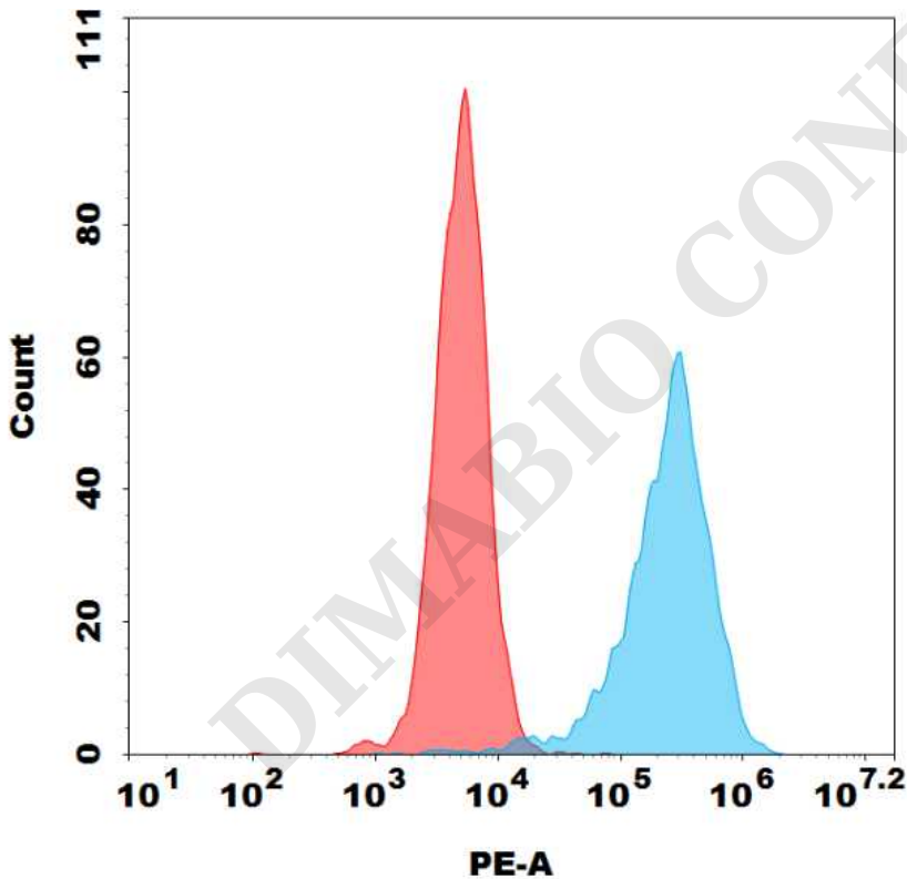
Figure 1. Flow cytometry analysis with 1 µl/test PE-conjugated Anti-CDH17(TORL-3-600 biosimilar) on SNU-5 cell line (Blue histogram) or 293T cell line (Red histogram).
