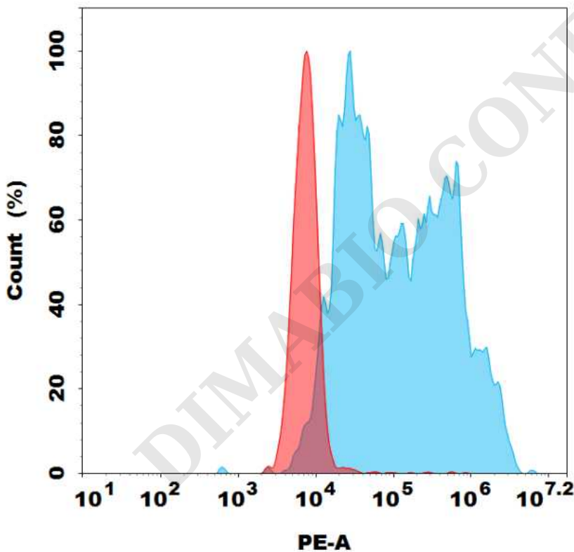
Figure 1. Flow cytometry analysis with 1 µl/test PE-conjugated Anti-PD-L1(durvalumab biosimilar ) mAb on HEK293 cells transfected with Human PD-L1 protein (Blue histogram) or HEK293 transfected with irrelevant protein (Red histogram).
